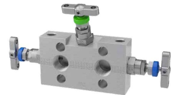
Example shown: 3-valve direct mount manifold with NPT connections and additional test/purge ports.
