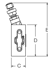
Example shown: 3-valve manifold with PTFree connect™ connection.
