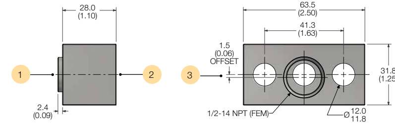
Example shown with traditional 1/2" NPT Fem. connection.
